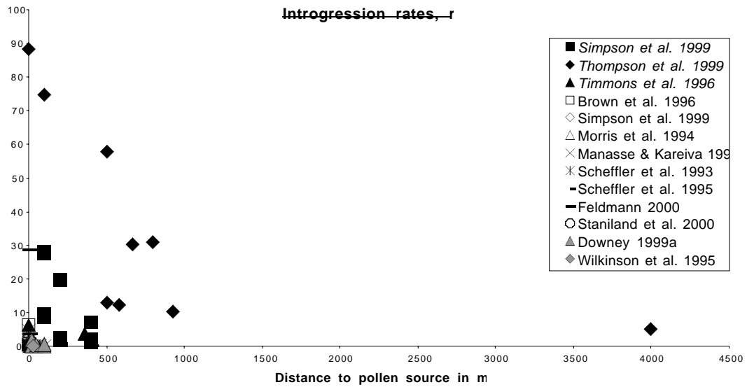
Fig. 10: Full overview of the determined introgression rates in rape as a function of distance to pollen source (various literature sources; studies shown in italics with a filled-in (black) key concern introgression in sterile male rape, while the other studies concern introgression in fertile male rape).
